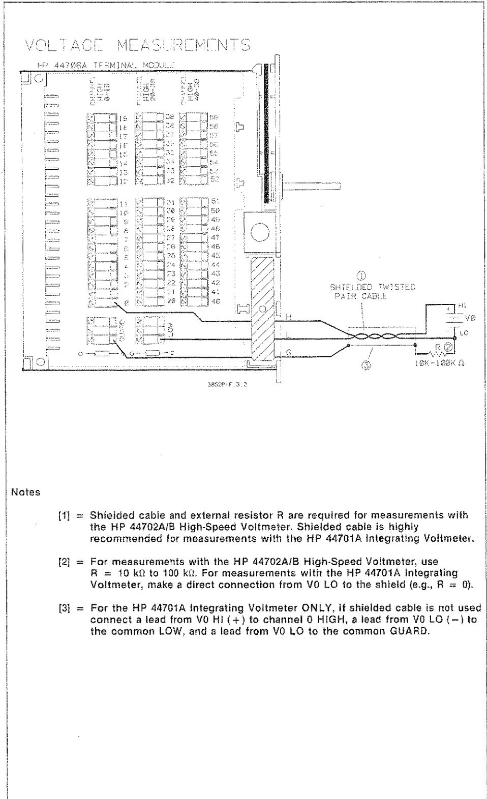
Figure 3-3. HP 44706A Voltage Connections
