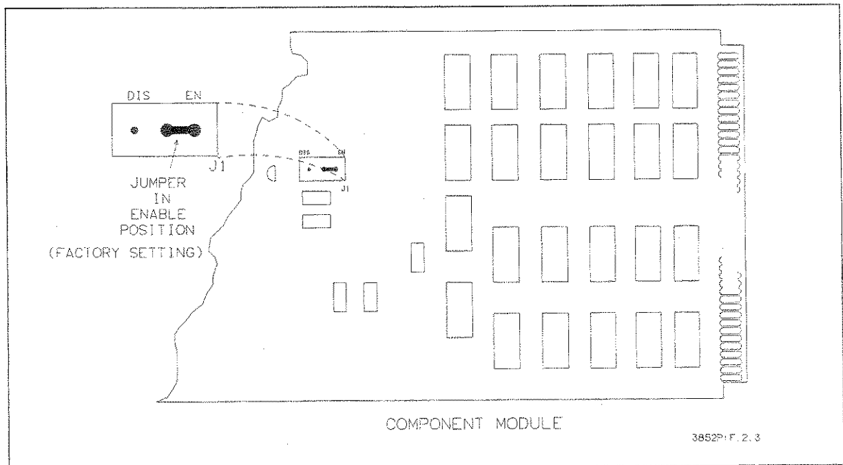
Figure 2-3. HP 44705A/44705H Isolation Jumper Configuration
