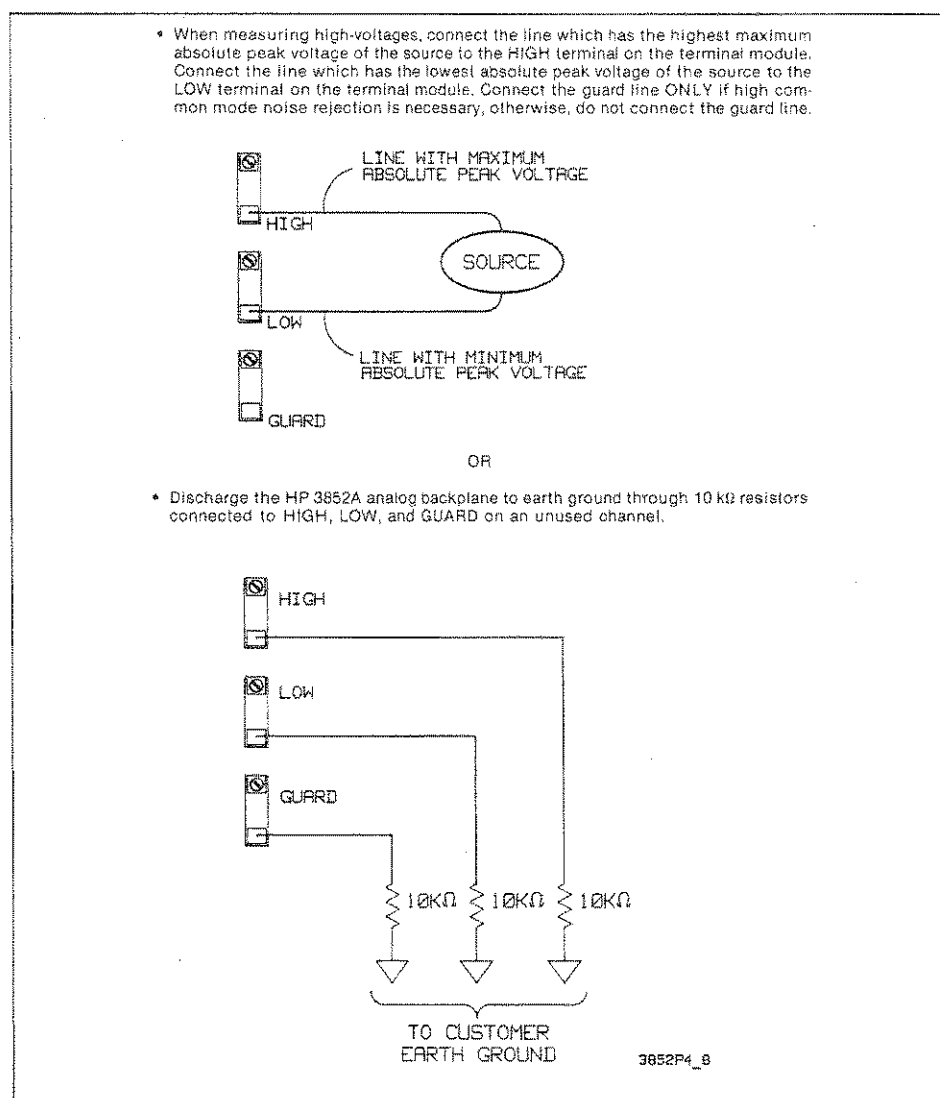
Figure 2-1. Discharging the HP 3852A Backplane
