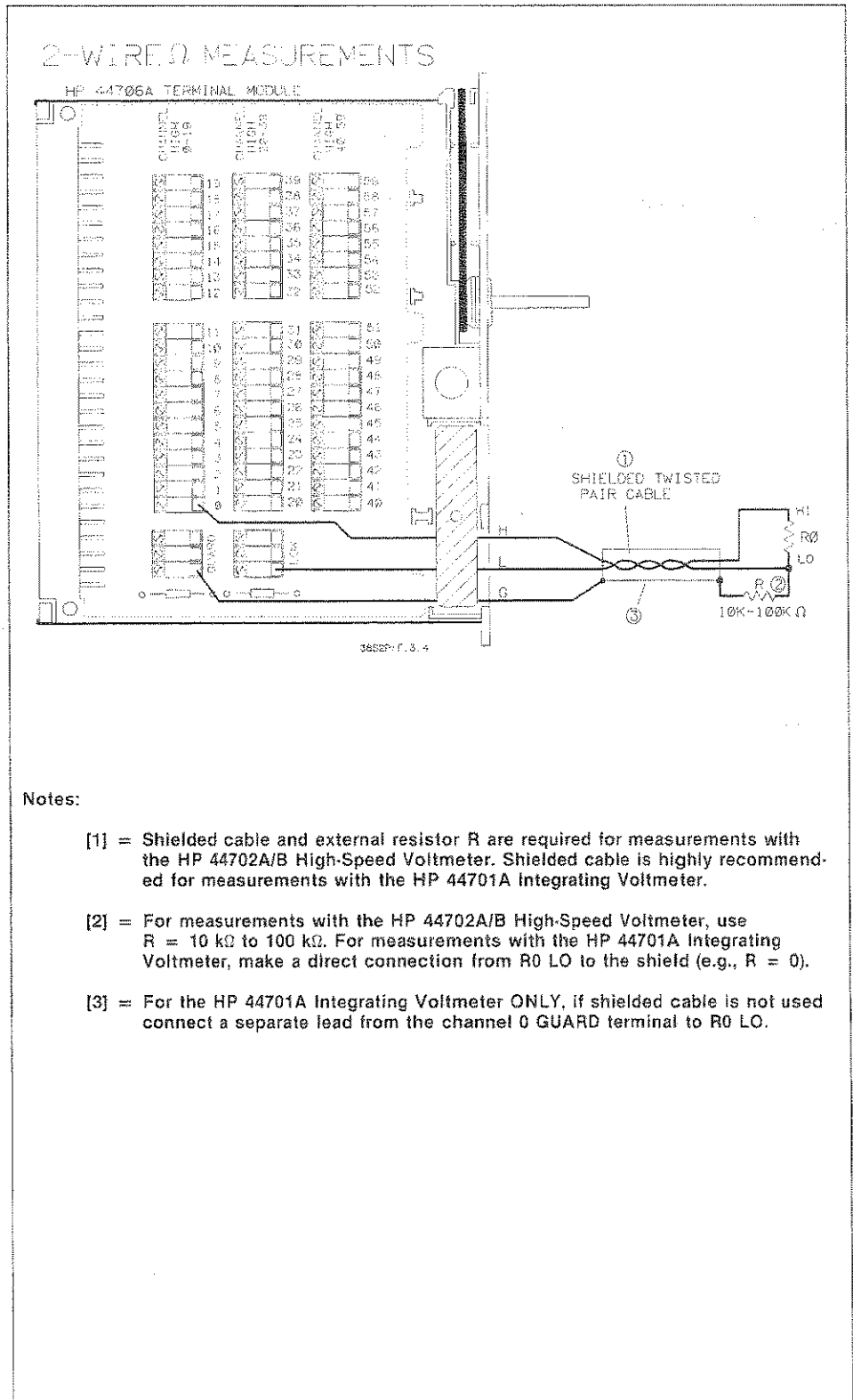
Figure 3-4. HP 44706A 2-Wire Ohms Connections
