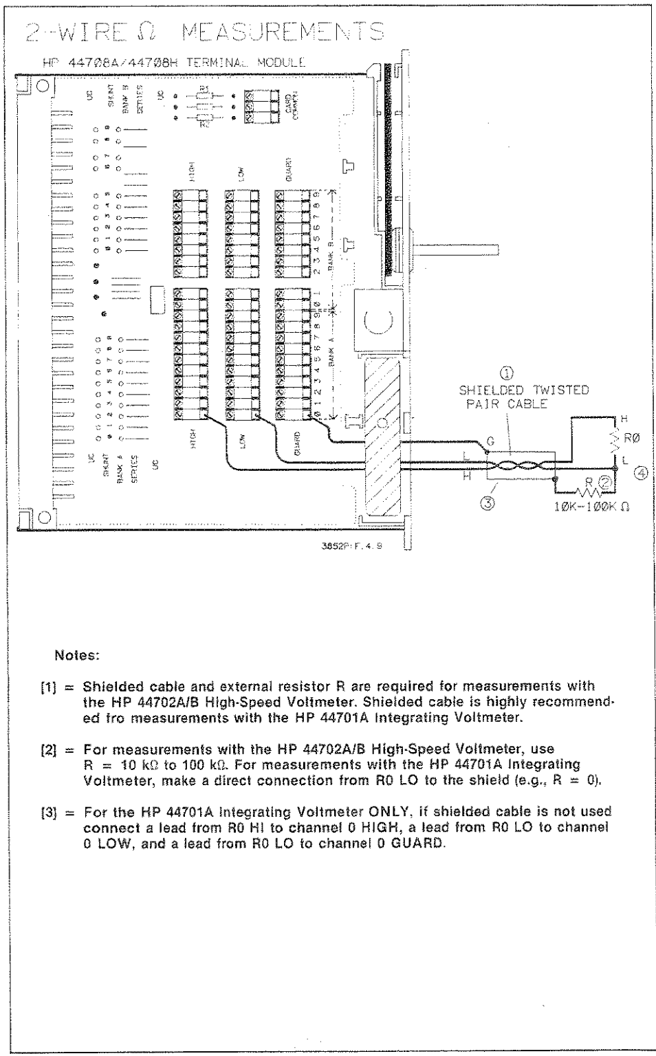
Figure 4-9. HP 44708A/44708H 2-Wire Ohms Connections
