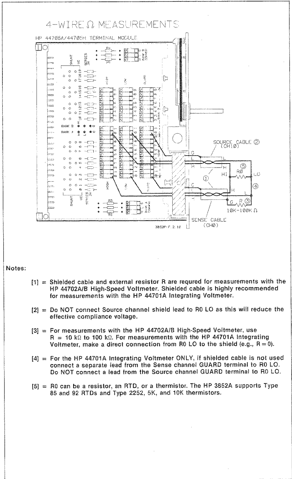
Figure 2-10. HP 44705A/44705H 4-Wire Ohms Connections
