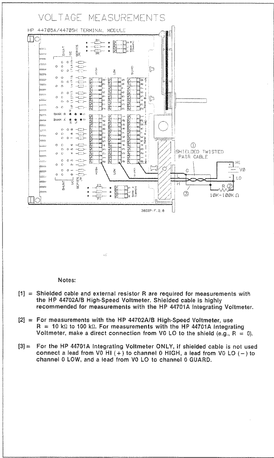
Figure 2-8. HP 44705A/44705H Voltage Connections
