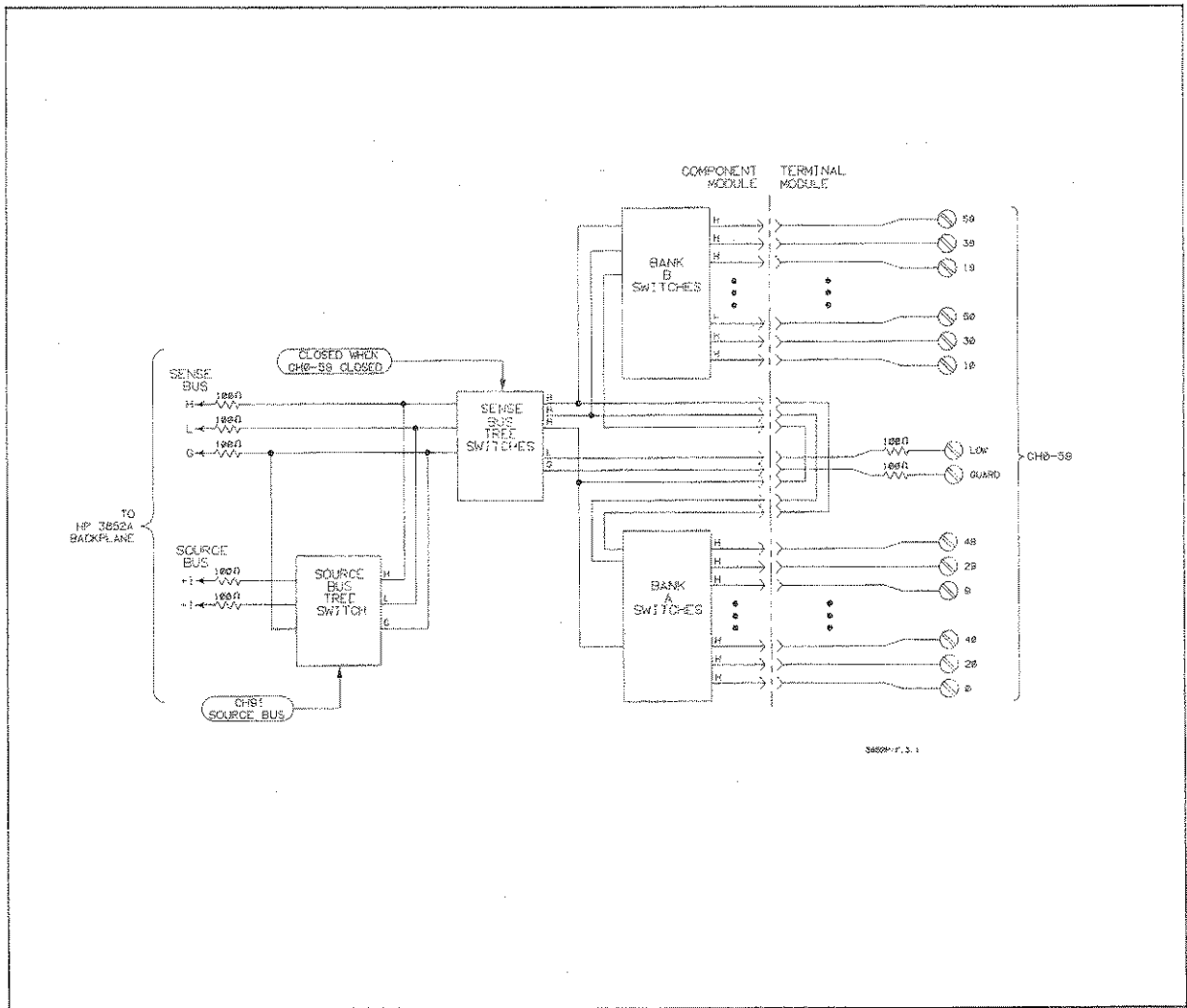
Figure 3-1. HP 44706A Block Diagram
