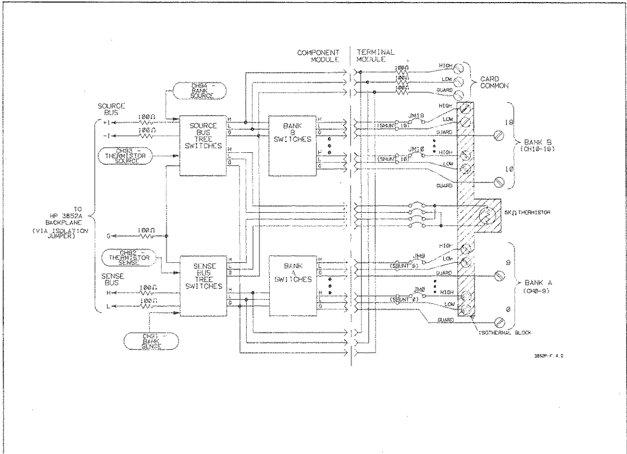
Figure 4-2. HP 44708A/44708H Block Diagram
